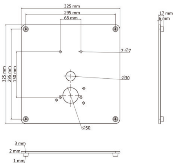
DS-KAB6-BASE (Optional)
