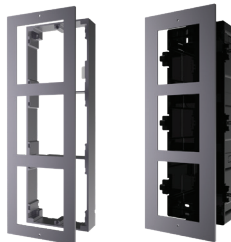
3 Modules Flush Mount Frame DS-KD-ACF3 DS-KD-ACF3/Plastic
