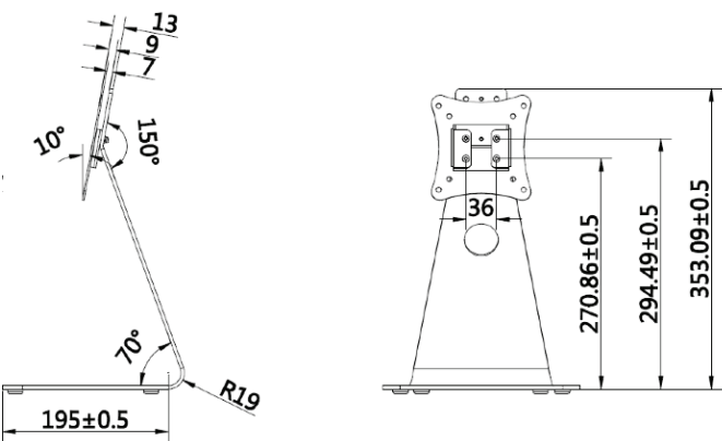
DS-DM0701BL (Optional)
