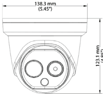
Thermal-Optical Turret
