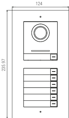
Dual Modules Flush Mounting
