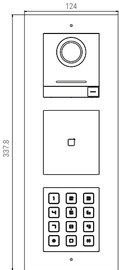
Three Modules Flush Mounting
