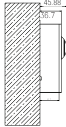
Single Module Surface Mounting
