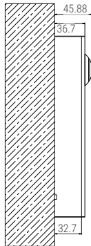
Dual Modules Surface Mounting
