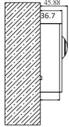
Single Module Surface Mounting
