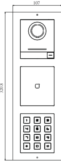
Three Modules Surface Mounting
