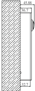
Dual Modules Surface Mounting
