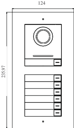
Dual Modules Flush Mounting
