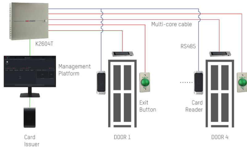
SOLUTION 1: Entrance by card, Exit by button
