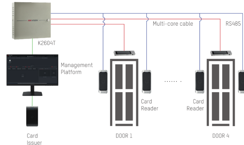
SOLUTION 2: Entrance by card, Exit by card
