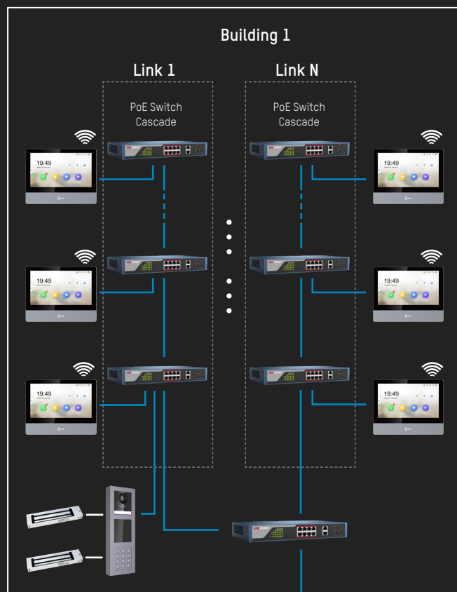
IP Solution
