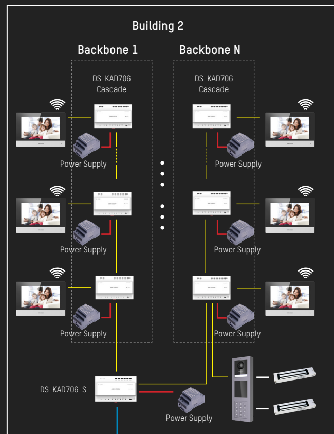
2-Wire Solution
