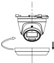
Figure 2-21 Remove the Trim Ring
