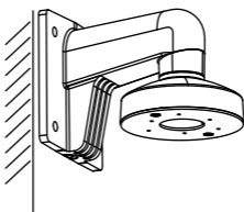
Figure 2-9 Fix the Wall Mount
