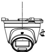
Figure 2-29 Loosen the Screw and Clip Plate
