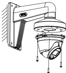
Figure 2-40 Install the Camera
