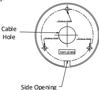
Figure 2-41 Drill Template
