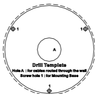
Figure 2-33 Drill Template
