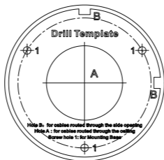
Figure 2-19 Drill Template
