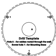
Figure 2-26 Drill Template
