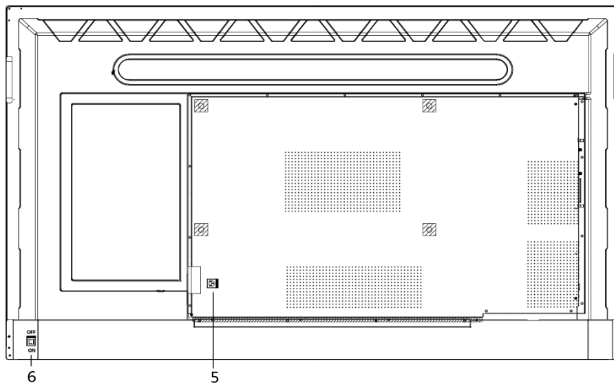
Figure 3-2 Back Panel
