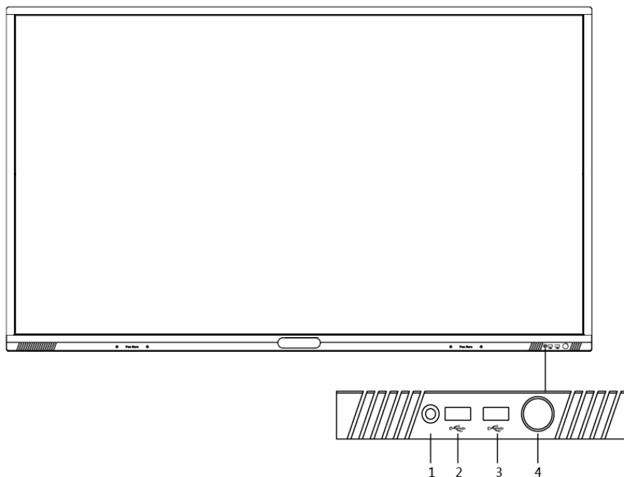
Figure 3-1 Front Panel
