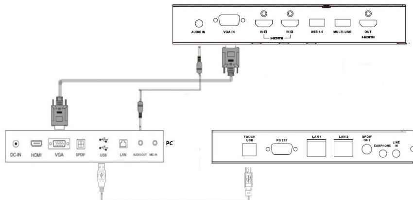
Figure 3-5 VGA Connection
