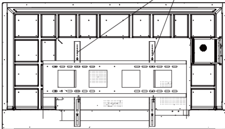
Figure 3-8 Wall Mount Front View
