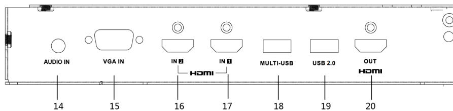
Figure 3-4 Interfaces on Back Panel Left
