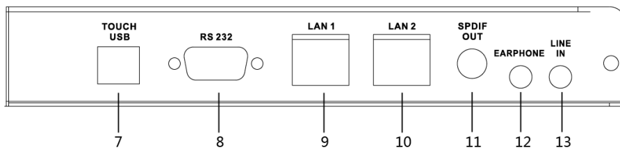
Figure 3-3 Interfaces on Back Panel Bottom
