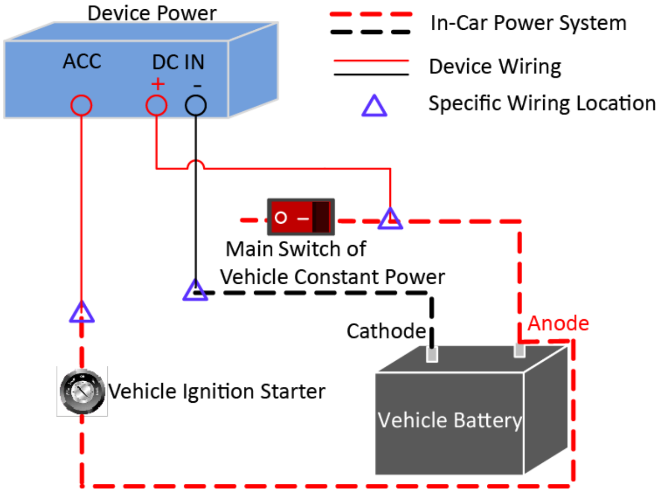
Figure 4-2 Power Wiring
