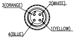
M12 MALE CONNECTOR PIN-OUT
