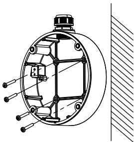
Figure 2-12 Secure the Junction Box' Camera Body to Ceiling/Wall 6. Combine the junction box's cover with the its body. 7. Repeat steps 5 to 8 of 2.1 Ceiling/Wall Mounting without Junction Box. to install the camera to the junction box.
