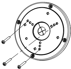
Figure 2-7 Install Turret Camera's Mounting Base
