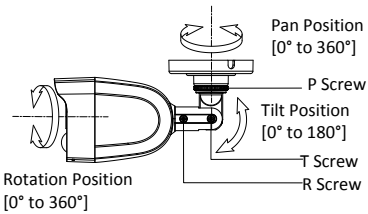
Figure 2-3 3-axis Adjustment
