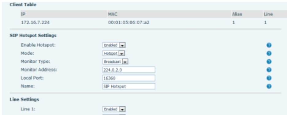
Picture 82 - SIP hotspot server configuration
