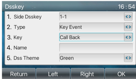
Picture 104 - DSS LCD key Page Configuration Screen
