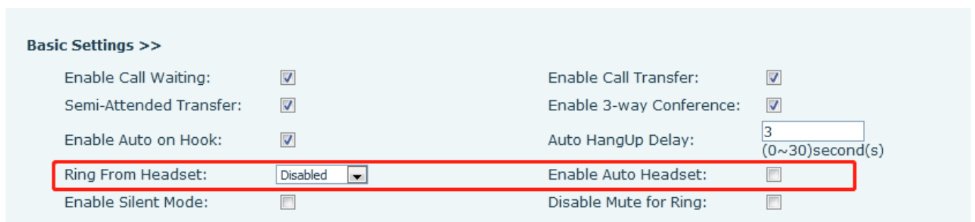
Picture 106 - Headset function settings
