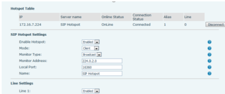
Picture 83 - SIP hotspot client configuration
