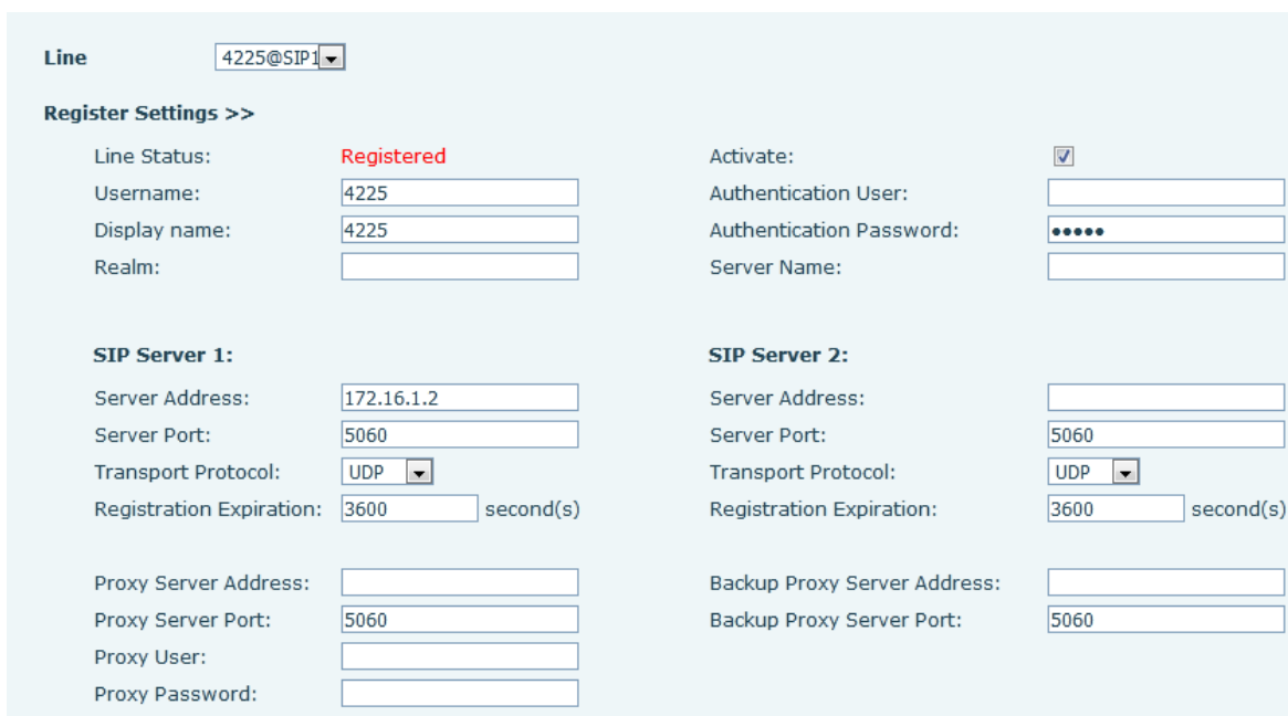
Picture 11 - Web SIP registration
