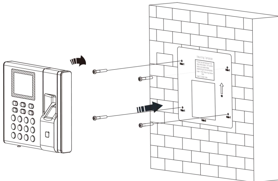
Figure 3-2 Install Device
