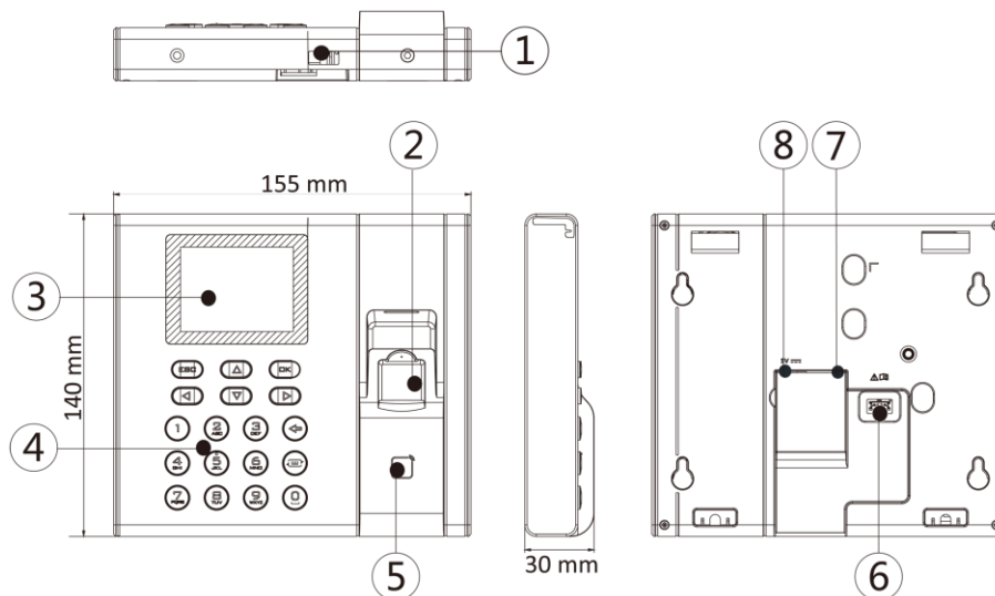
Figure 2-1 Device Appearance
