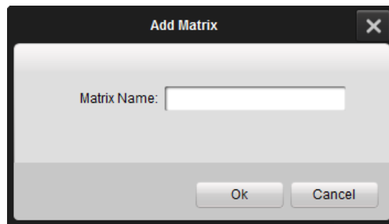
Figure 3. 28 Add Matrix
