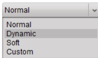
Figure 3. 25 Image Mode
