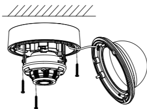
Figure 2-9 Attach the Back Box
