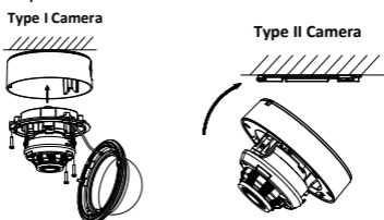
Figure 2-3 Fix the camera to the Ceiling
