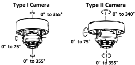
Figure 2-4 3-Axis Adjustment
