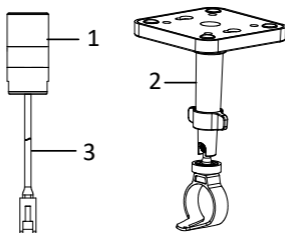
Figure 1-14 Tube Lens
