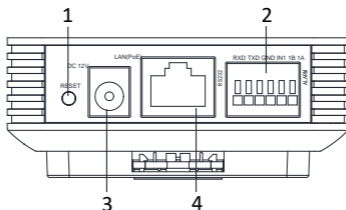
Figure 1-9 Type I Covert Camera Rear Panel
