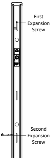
Figure 2-21 Secure Base on Wall
