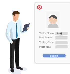
Easy Registration
