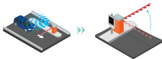
Vehicle Detection
