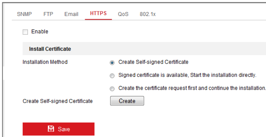
Figure 6-11 HTTPS Configuration Interface
