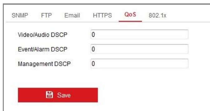
Figure 6-14 QoS Settings
