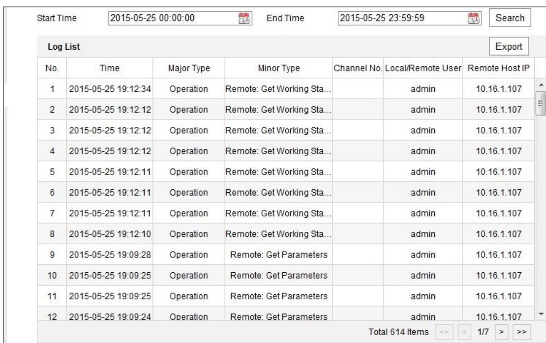
Figure 5-12 Log Searching
