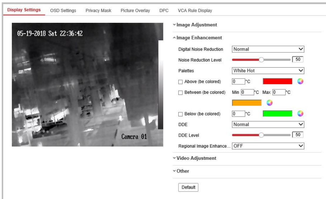
Figure 8-6 Image Enhancement
