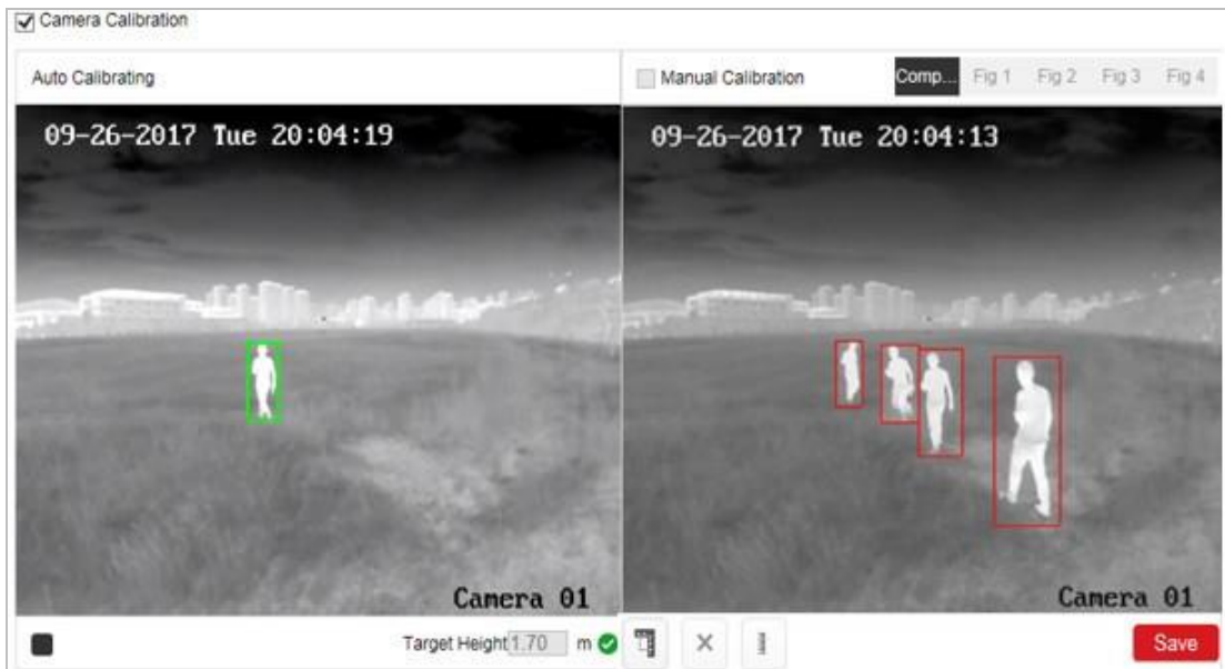
Figure 9-16 Auto Calibration
