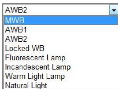
Figure 8-4 White Balance
