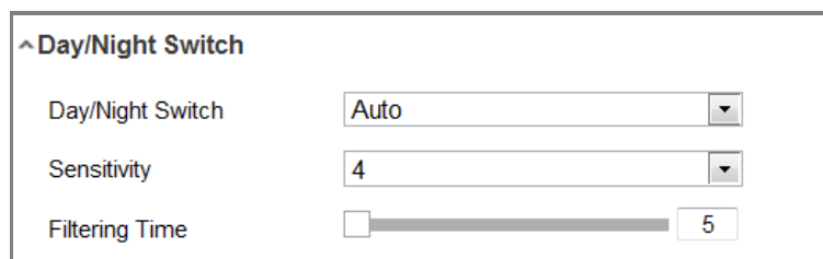
Figure 8-3 Day/Night Switch
