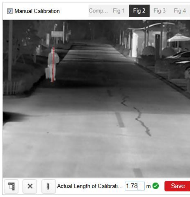
Figure 9-18 Manual Calibration (2)
