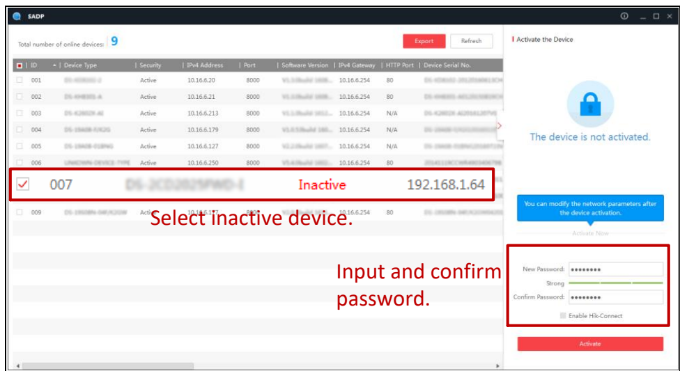
Figure 2-4 SADP Interface
