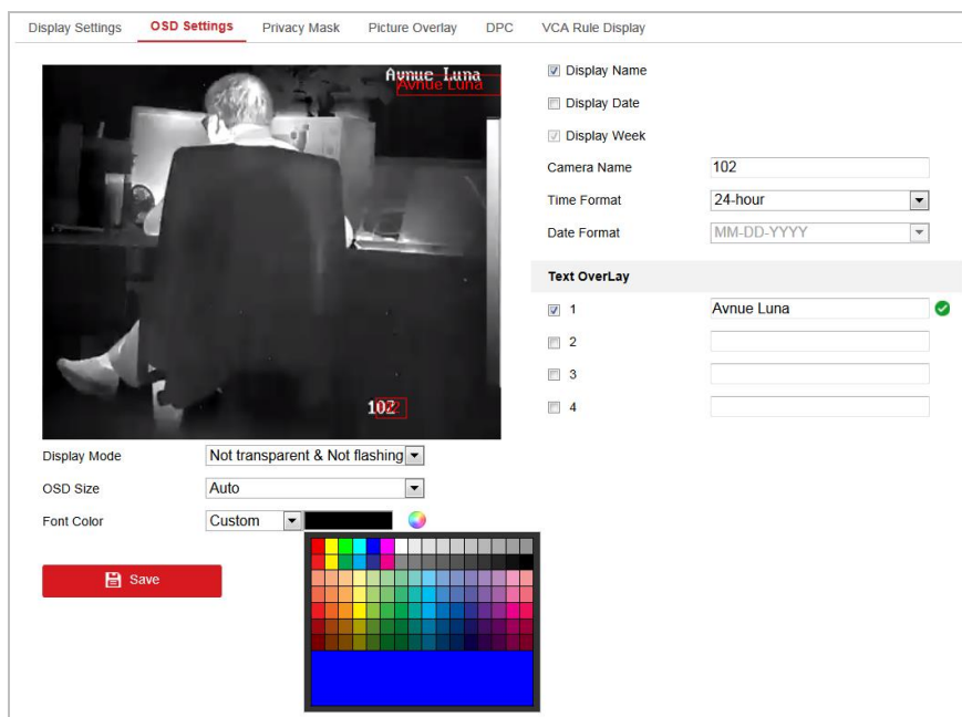
Figure 8-7 OSD Settings
