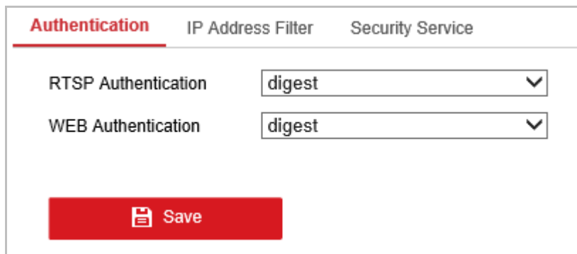
Figure 5-15 RTSP / WEB Authentication
