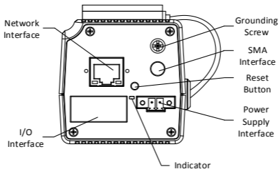
Figure 1-2 Rear Panel
