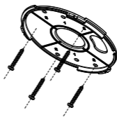
Figure 2. 10 Attach the Back Box/Base Plate
