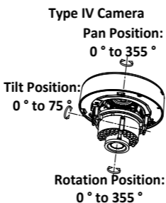
Figure 2. 12 3-axis Adjustment
