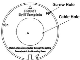
Figure 2. 4 Drill Template
