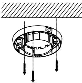
Figure 2. 6 Fix the Mounting Base on the Ceiling
