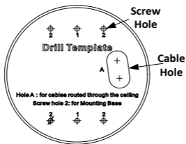
Figure 2. 9 The Drill Template
