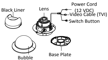
Figure 1. 4 Type IV Camera Overview
