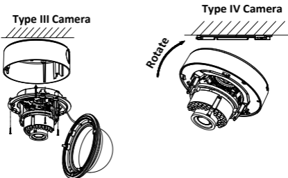
Figure 2. 11 Fix the Camera to the Ceiling
