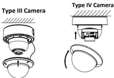
Figure 2. 13 Finish the Installation
