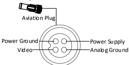
Figure 1-2 Interfaces of Aviation Plug
