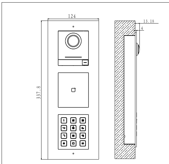
Three Modules Flush Mounting
