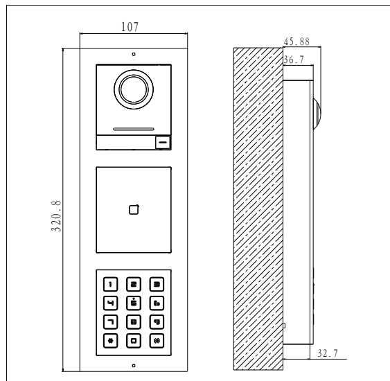
Three Modules Surface Mounting
