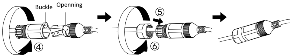
Figure 4-3 Complete Installation
