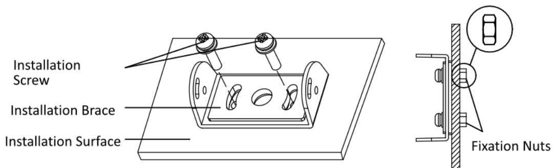
Figure 1-27 Installing Support
