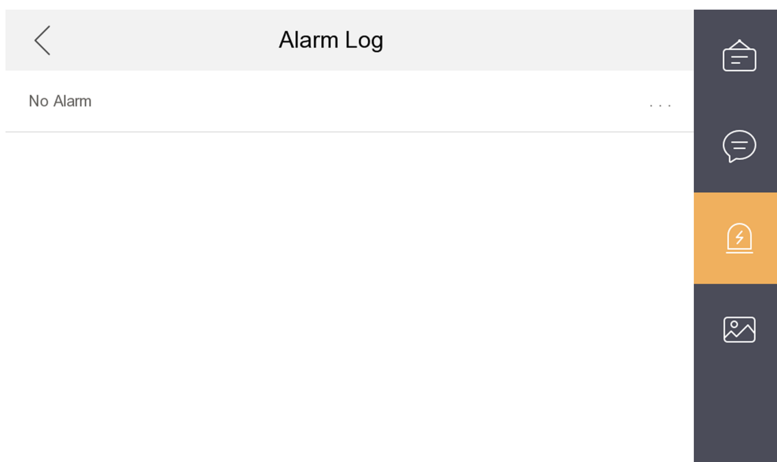
Figure 2-8 Alarm Logs
