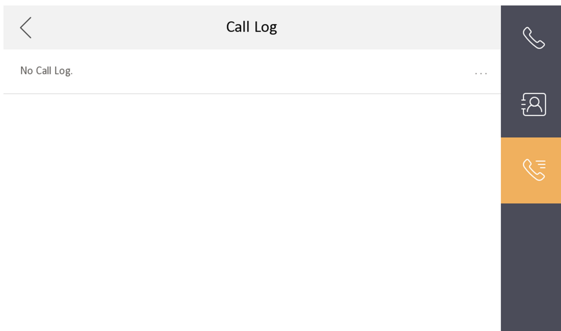
Figure 2-3 Call Logs
