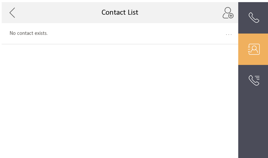
Figure 2-1 Contact List
