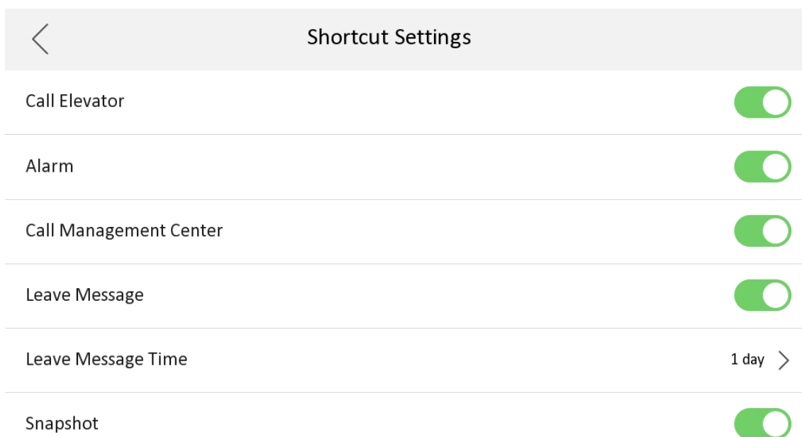
Figure 2-7 Call Elevator
