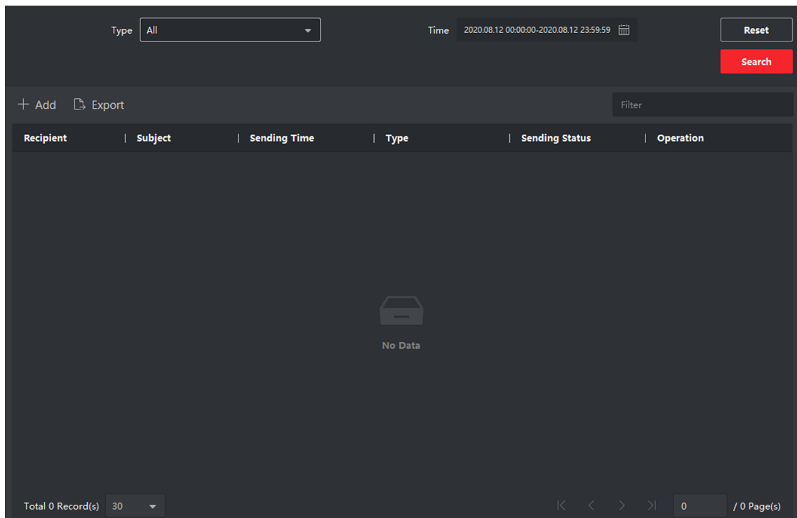
Figure 3-4 Release Notice
