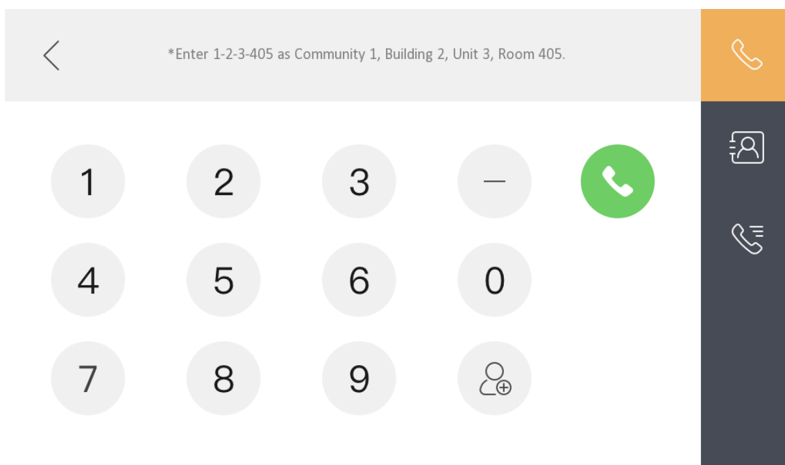
Figure 2-2 Call Resident
