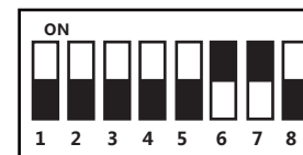
DIP Switch of Wiegand 26 Protocol
