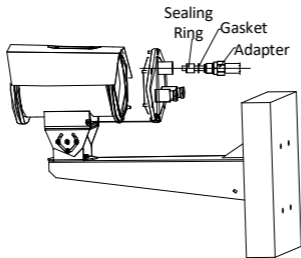
Figure 3-10 Secure Adapter to the Back Cover
