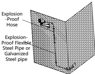
Figure 3-12 Route Cables
