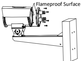
Figure 3-7 Remove the Back Cover
