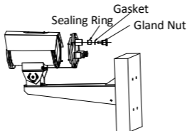
Figure 3-8 Loosen the Gland Nut
