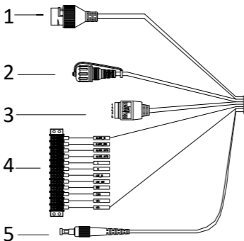
Figure 2-2 Overview of Cables
